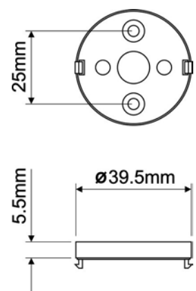
Base plate
